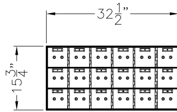
MODEL 515-18 (18) 5 x 5 OPENINGS
