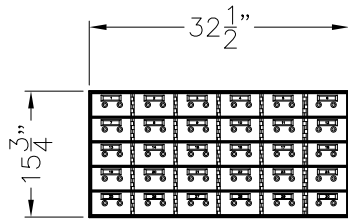
MODEL 515-30 (30) 3 x 5 OPENINGS
