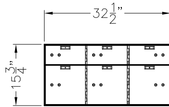
MODEL 515-6 (3) 5 x 10 OPENINGS (3) 10 x 10 OPENINGS
