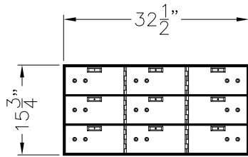
MODEL 515-9 (9) 5 x 10 OPENINGS
