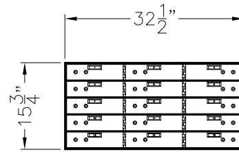
MODEL 515-15 (15) 3 x 10 OPENINGS
