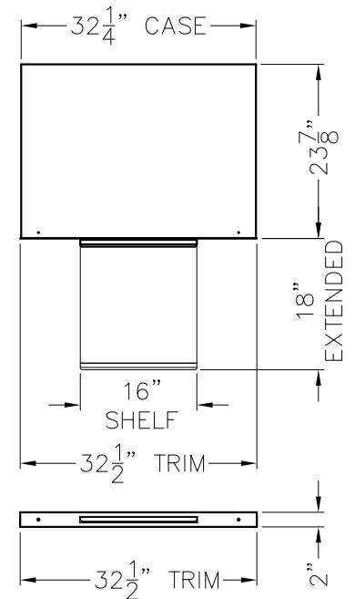
MODEL 522-9200 PULL SHELF ASSEMBLY
