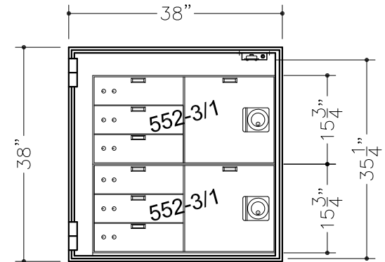
(6) 5x16 TELLER LOCKERS (2) 15x16 CASH LOCKERS (1) BASE (WELD-IN)
