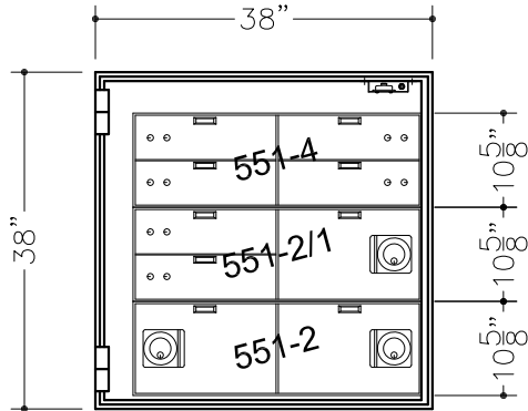
(6) 5x16 TELLER LOCKERS (3) 10x16 CASH LOCKERS (1) BASE (WELD-IN)
