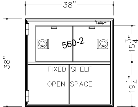
(2) 15x16 CASH LOCKERS (1) FIXED SHELF (WELD-IN)
