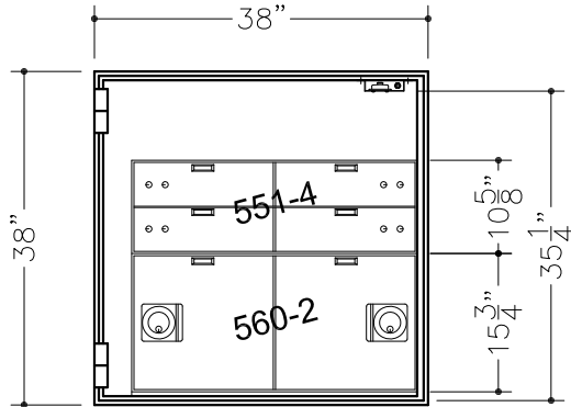
(4) 5x16 TELLER LOCKERS (2) 15x16 CASH LOCKERS (1) BASE (WELD-IN)
