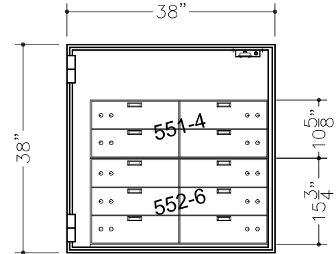
(10) 5x16 TELLER LOCKERS (1) BASE (WELD-IN)
