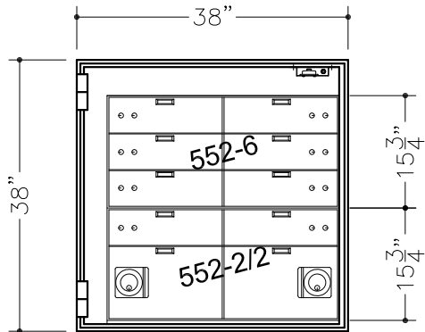
(8) 5x16 TELLER LOCKERS (2) 10x16 CASH LOCKERS (1) BASE (WELD-IN)
