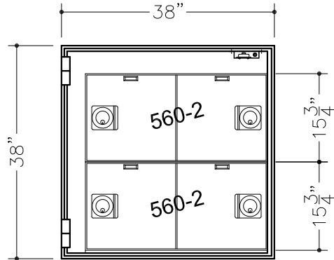
(4) 15x16 CASH LOCKERS (1) BASE (WELD-IN)
