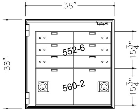
(6) 5x16 TELLER LOCKERS (2) 15x16 CASH LOCKERS (1) BASE (WELD-IN)
