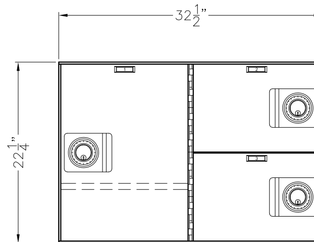
MODEL 563-3 (1) 22 x16 OPENING WITH ADJ SHELF (2) 10x16 OPENINGS
