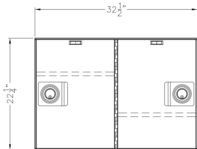
MODEL 563-2 (2) 22x16 OPENINGS WITH ADJ SHELVES
