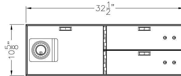
MODEL 551-1/2 (1) 10x16 OPENING (2) 5x16 OPENINGS
