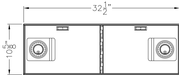
MODEL 551-2 (2) 10x16 OPENINGS
