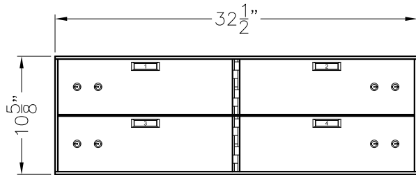
MODEL 551-4 (4) 5x16 OPENINGS
