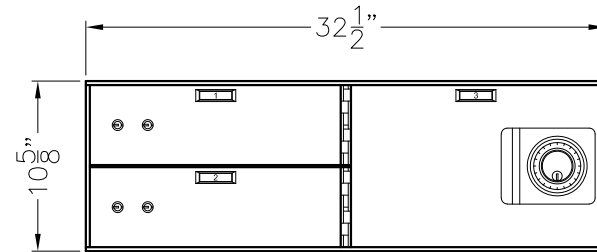
MODEL 551-2/1 (2) 5x16 OPENINGS (1) 10x16 OPENING
