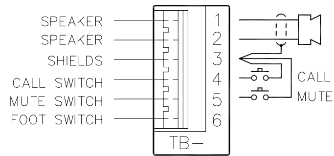
TERMINAL BLOCK DETAIL (TB-1 & TB-2)
